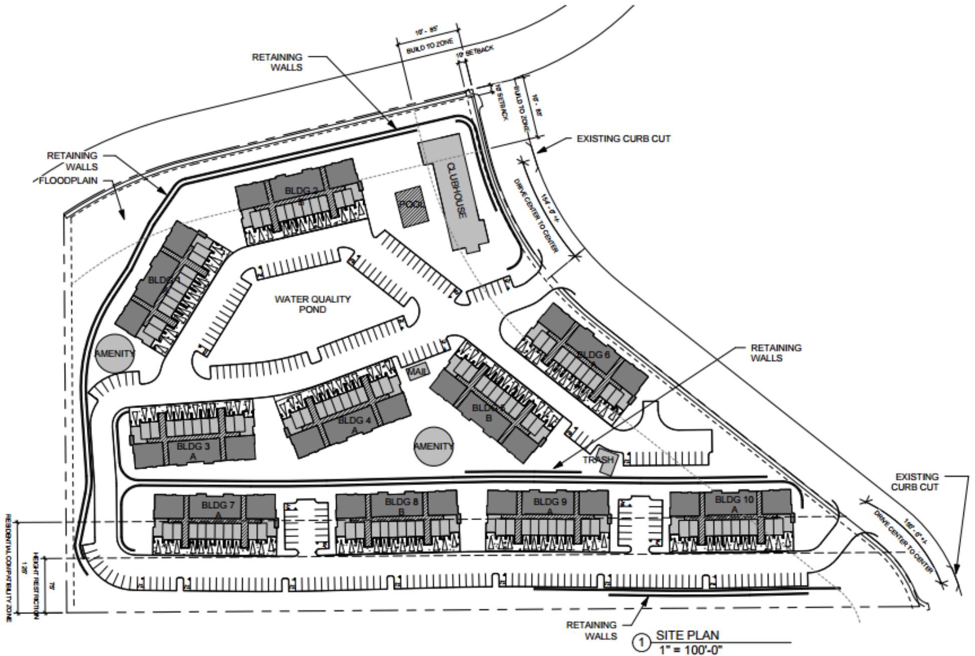
This diagram looks east and shows 4 25-unit buildings and parking along the back of Alkire houses with the rest of the development reaching to Safeway shipping center. There are two entrances on Mississippi Ct.
